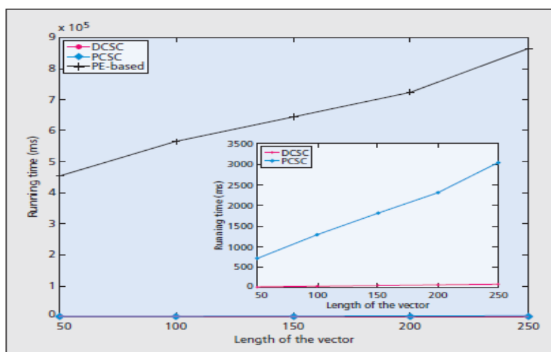
Fig 2. The Computation Overheads Of DCSC
