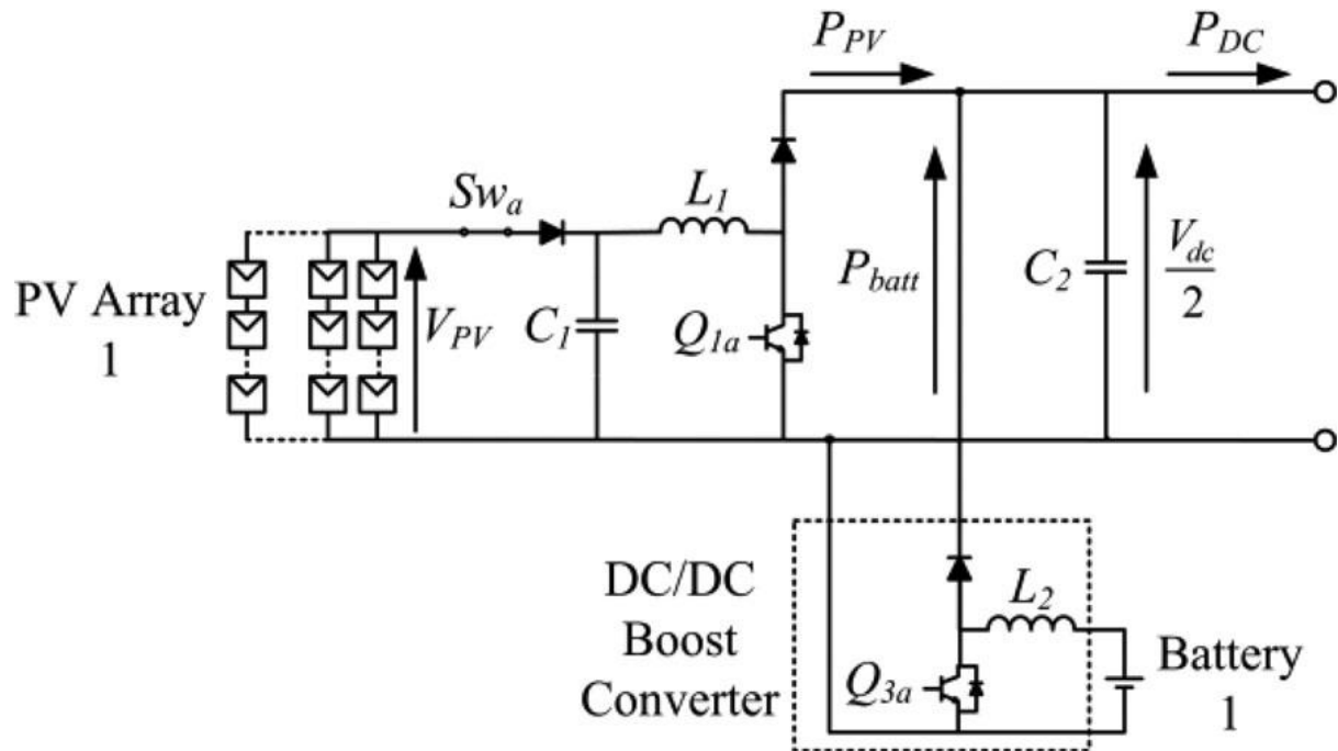
Fig7 Equivalent circuit during discharging operation
