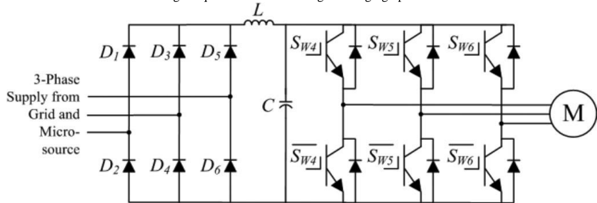
Fig. 8. Configuration of a 15kVA three-phase ASD.
