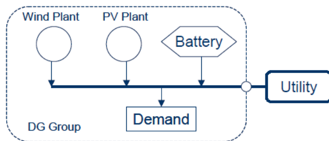
Fig 9 Typical DG grouping
