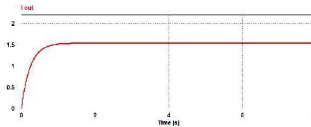
Figure 13: (d) Current Output of the Boost Converter ( I_{out} = 1.49 A)
