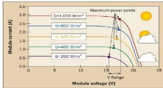
Figure 4: Effect on I-V Char. Change of Radiation [3]
