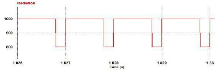
Figure 9: (a) Radiation from 1000 W/m 2 to 800 W/m 2
