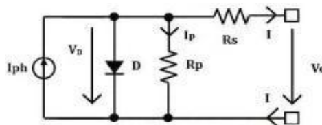
Figure 1: Equivalent Circuit of a PV Cell[4]
