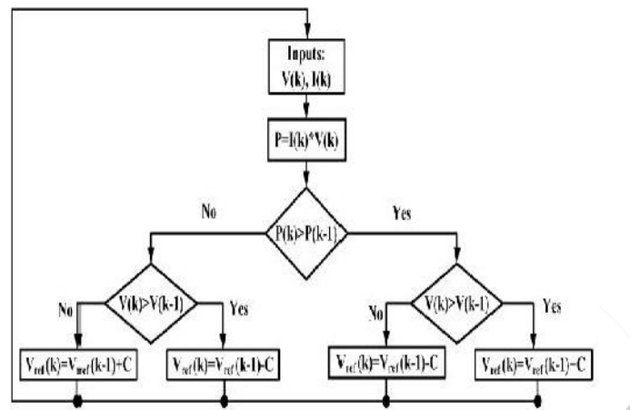
Figure 7: The Flowchart of the P&O Algorithm
