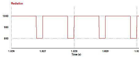
Figure 13: (a) Radiation from 1000 W/m 2 to 800 W/m 2
