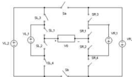
Figure 1. Circuit Diagram of Proposed Cascaded 31-level Inverter
