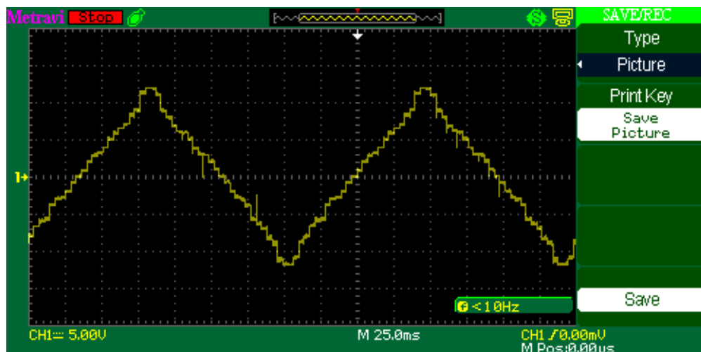
Figure 8 output voltage of cascaded H-bridge multilevel inverter (31-levels)
