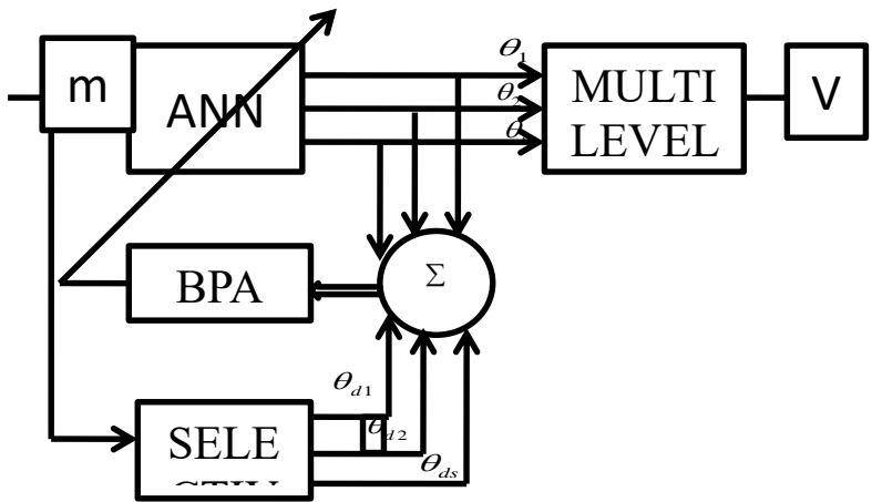
Figure 3. Back Propagation Algorithm
