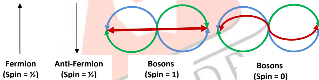
Fig. 6 Nature of Fermion and Bosons Particles
