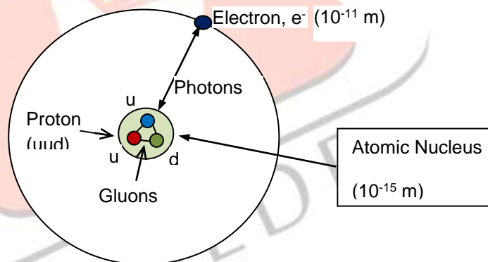
Fig. 1 Hydrogen Atom
