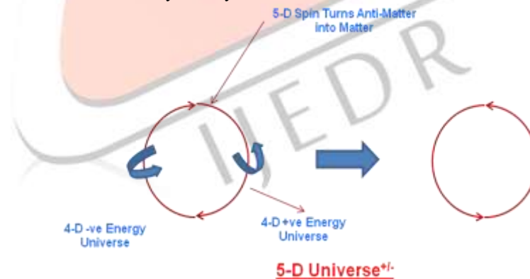
Fig. 11 Matter – Antimatter Asymmetry and Spin in 5-D Universe
