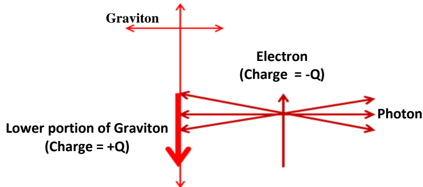
Fig. 8 Relation between Electron and Graviton in an Atom
