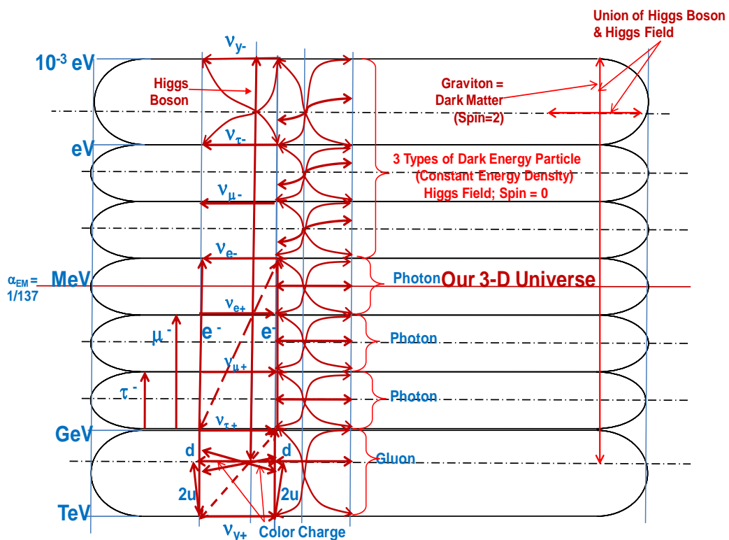
Fig. 7 Graviton, Dark Matter and 3 Types of Dark Energy
