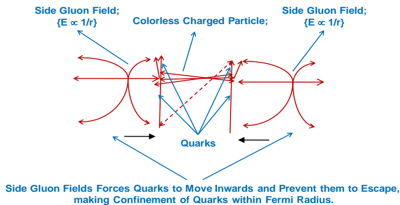
Fig. 5 Quark Confinement And Side Gluons
