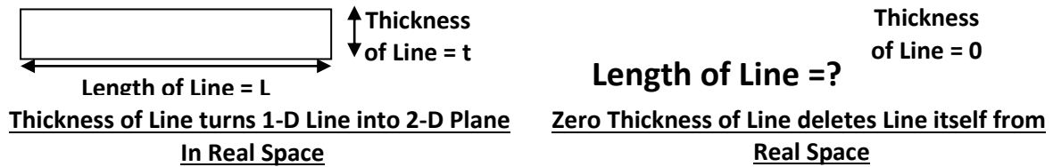
Fig. 2 Nature of One Dimensional Line
