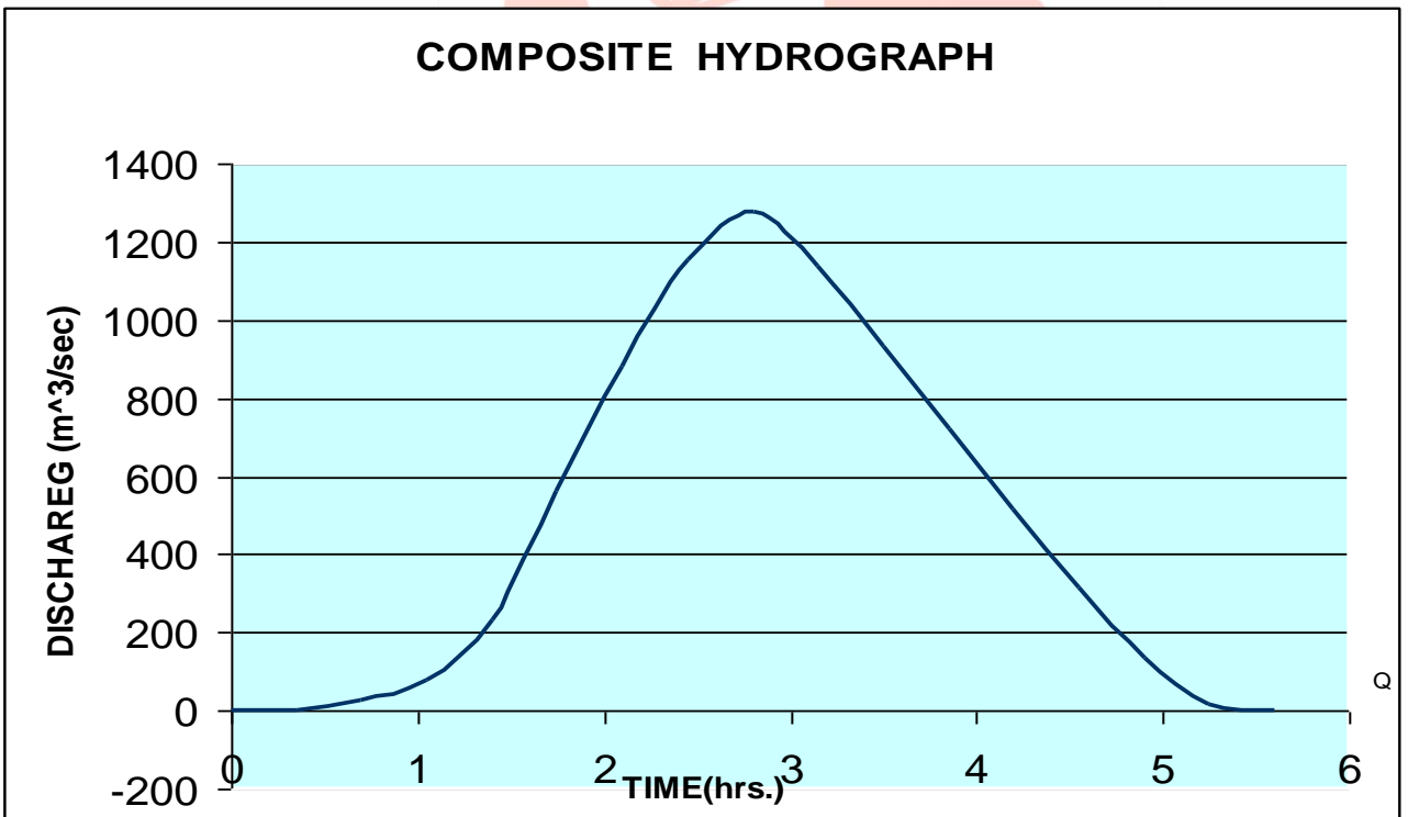
Figure 2 Composite Hydrograph
