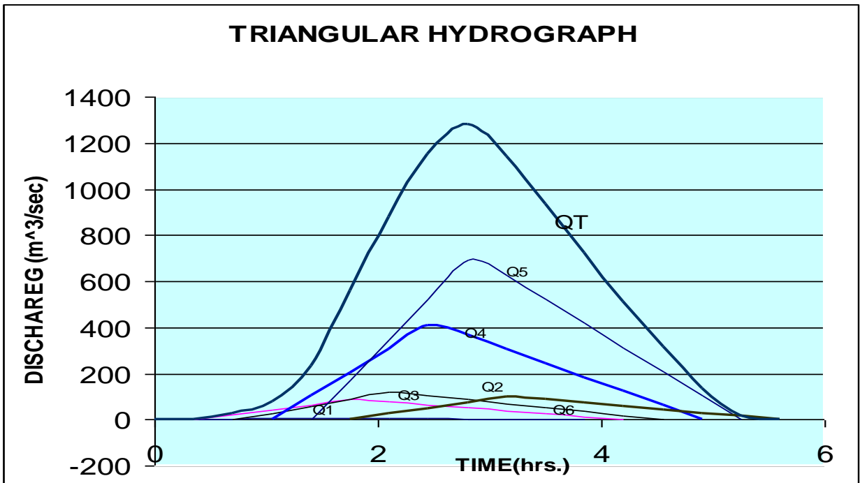
Figure 1 Triangular Hydrograph
